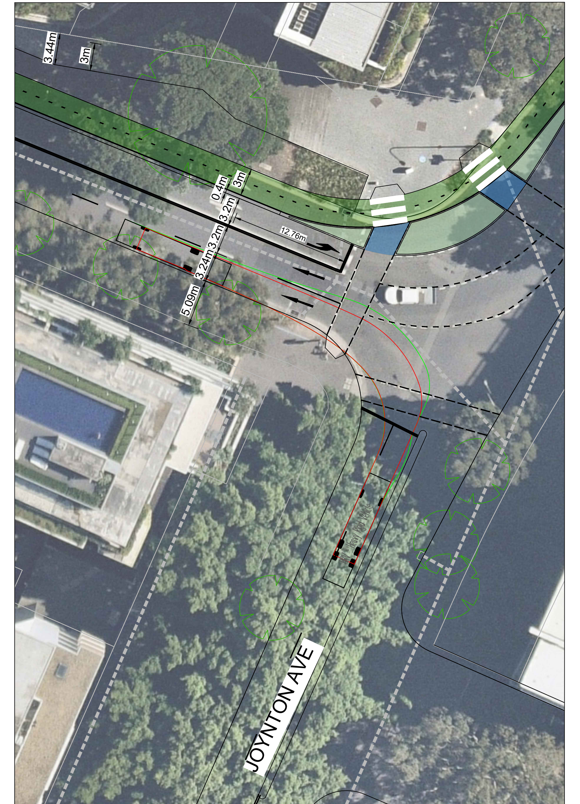
HEAVY RIGID VEHICLE (12.5m) SCALE 1:250
